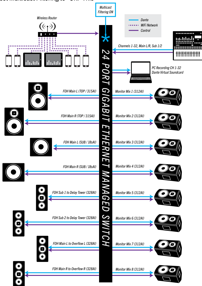
Managed Switch Network
