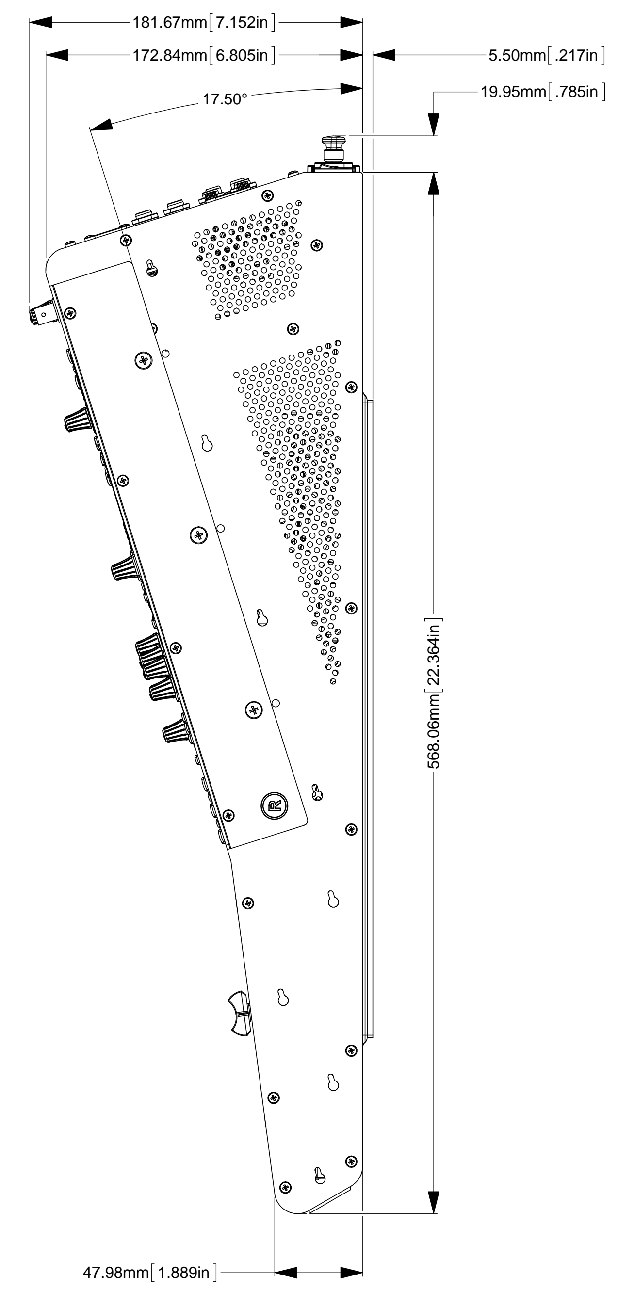
RIGHT VIEW SCALE 1:2
