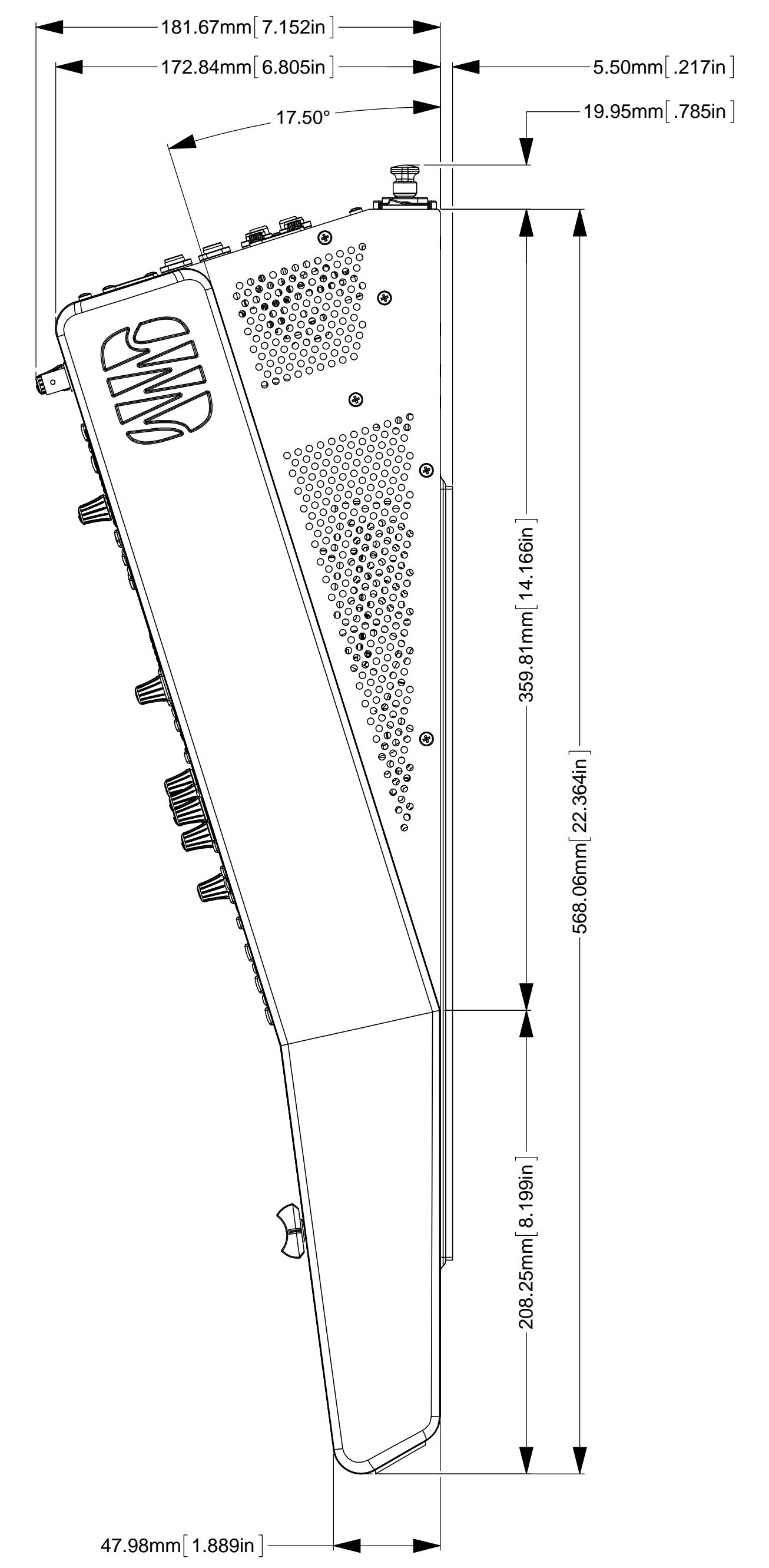
RIGHT VIEW SCALE 1:2
