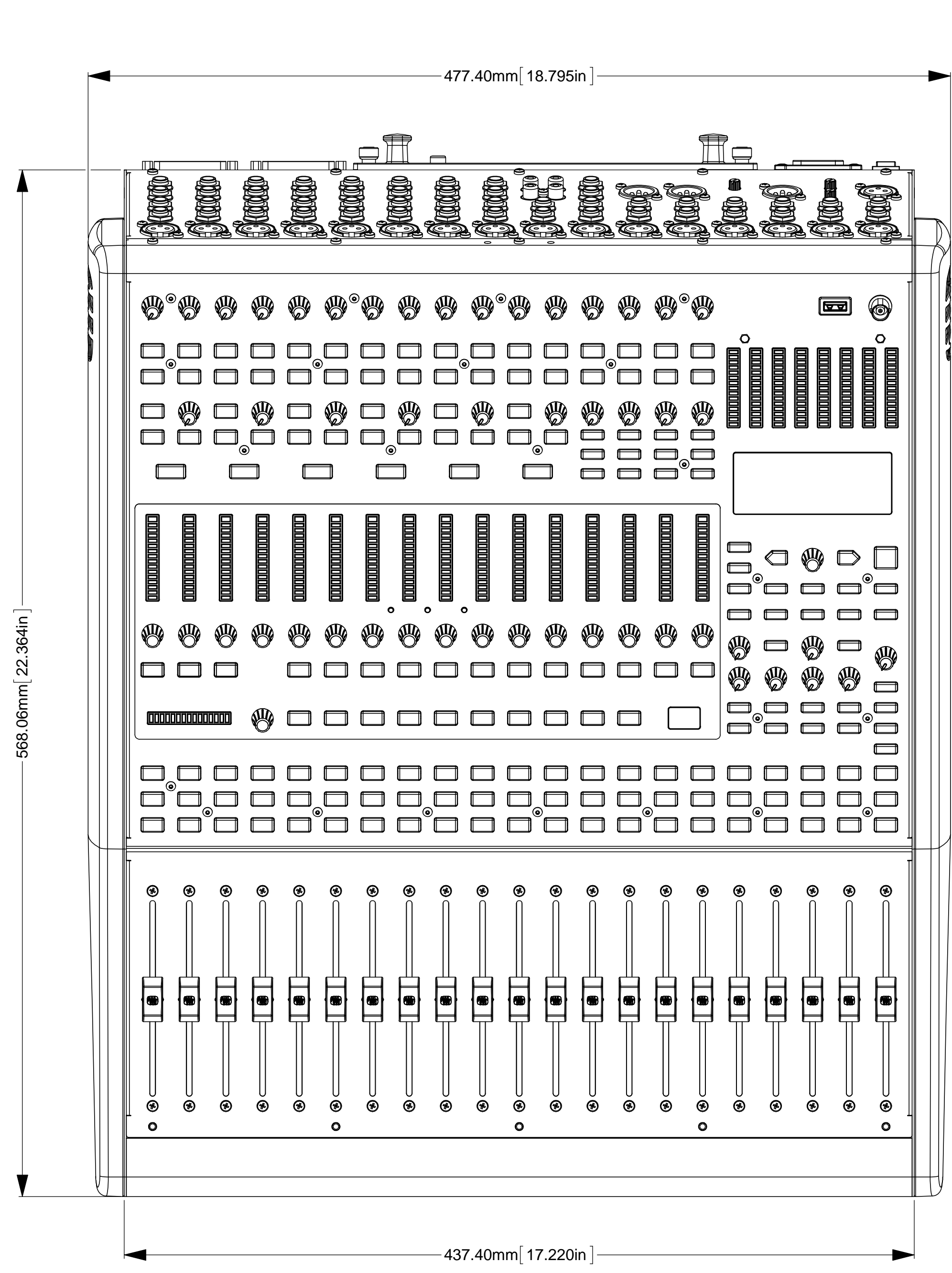
TOP VIEW SCALE 1:2
