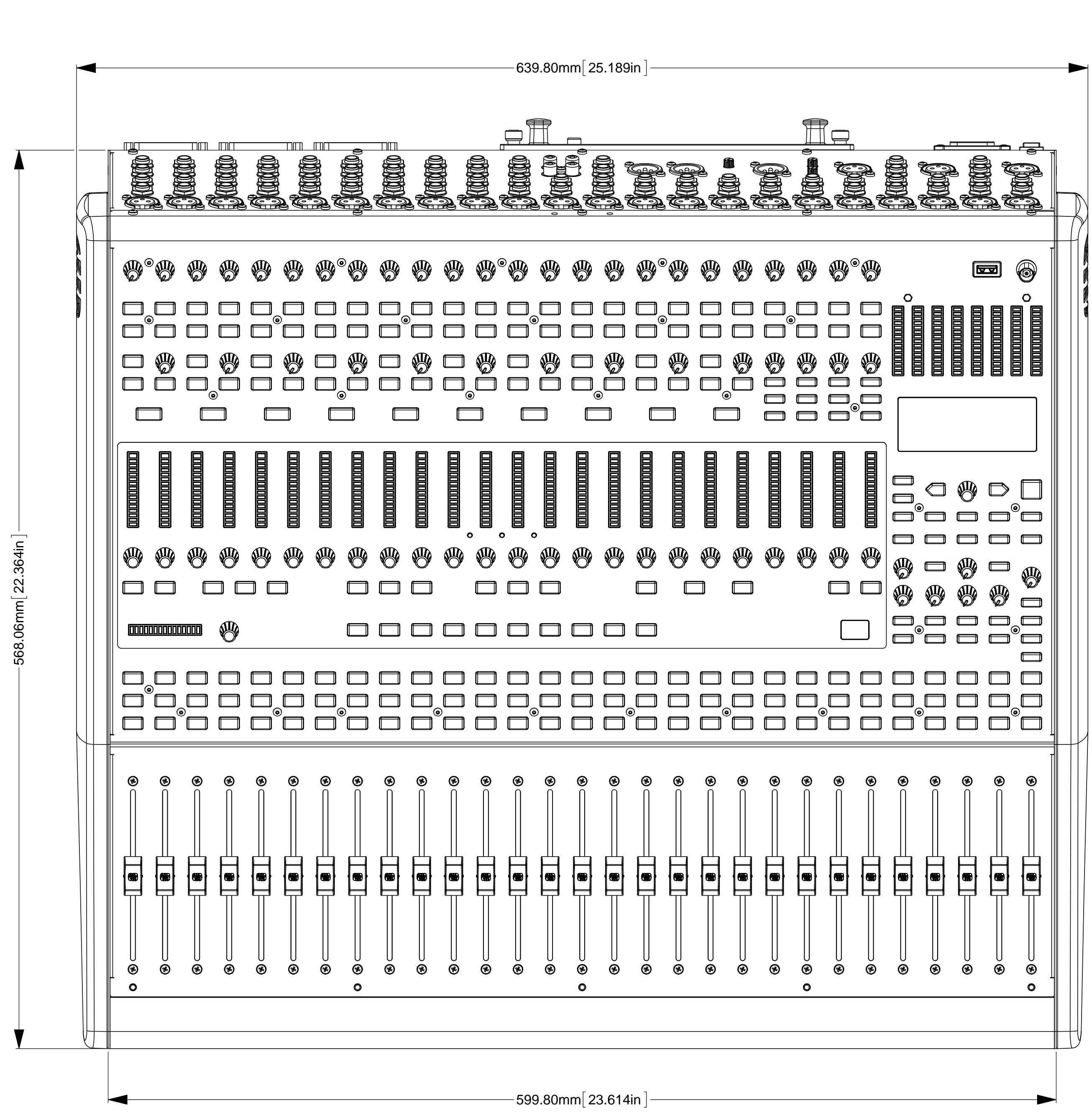
TOP VIEW SCALE 1:2
