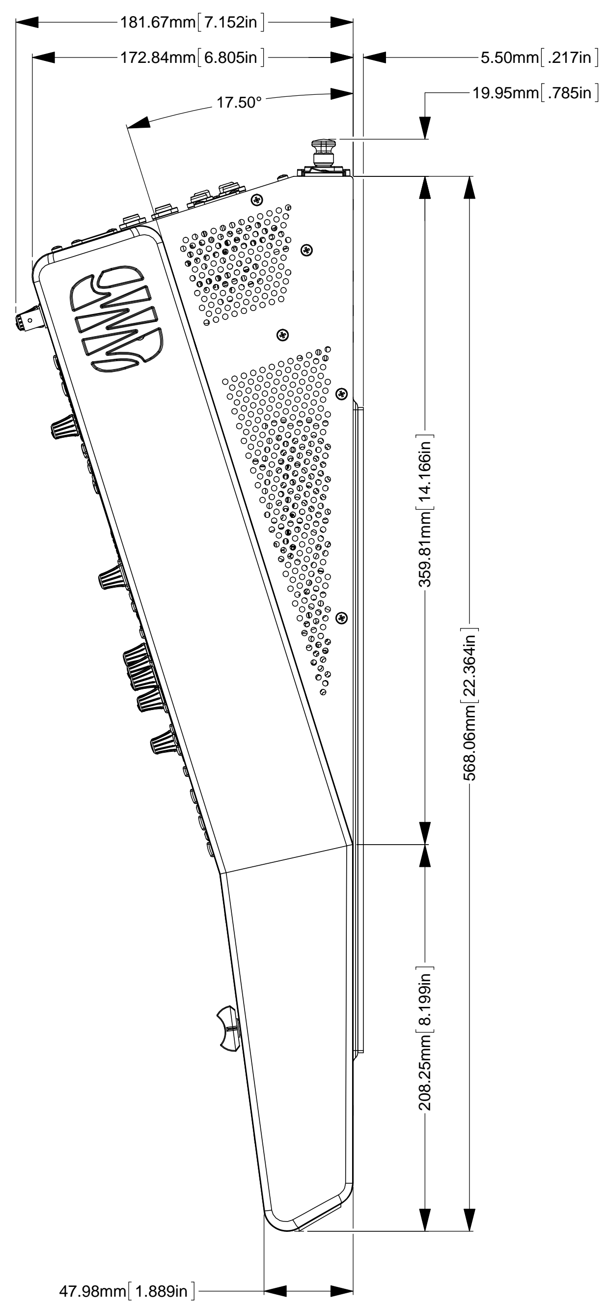
RIGHT VIEW SCALE 1:2
